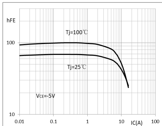
hFE - I_C (BA16P25A)
