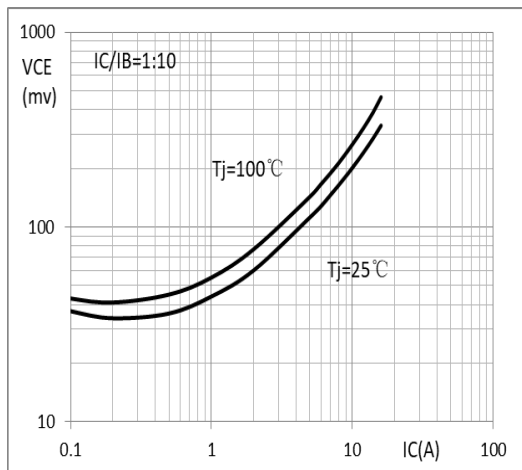
V_{CE(sat)} - I_C (BA16N25A)
