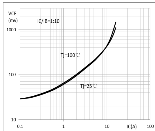
V_{CE(sat)} - I_C (BA16P25A)
